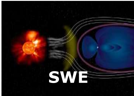
Space Weather
